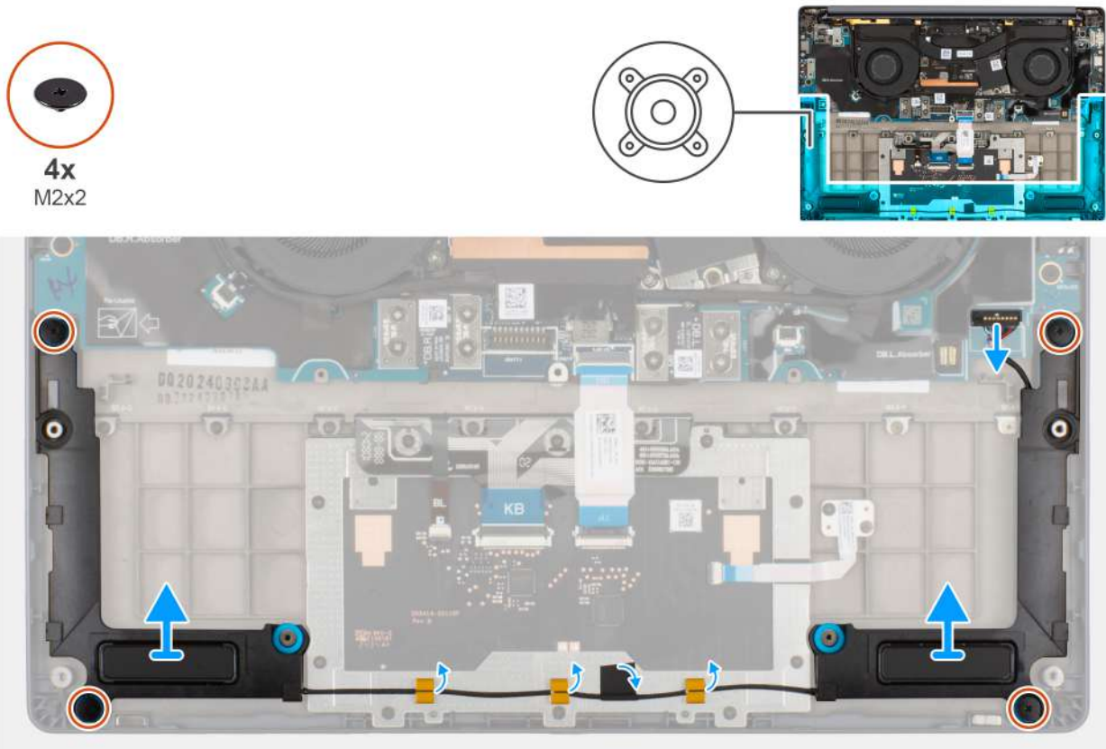
Figure 32. Removing the speakers without antenna (WLAN configuration)
