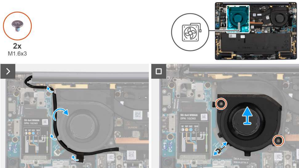
Figure 30. Removing the right fan
