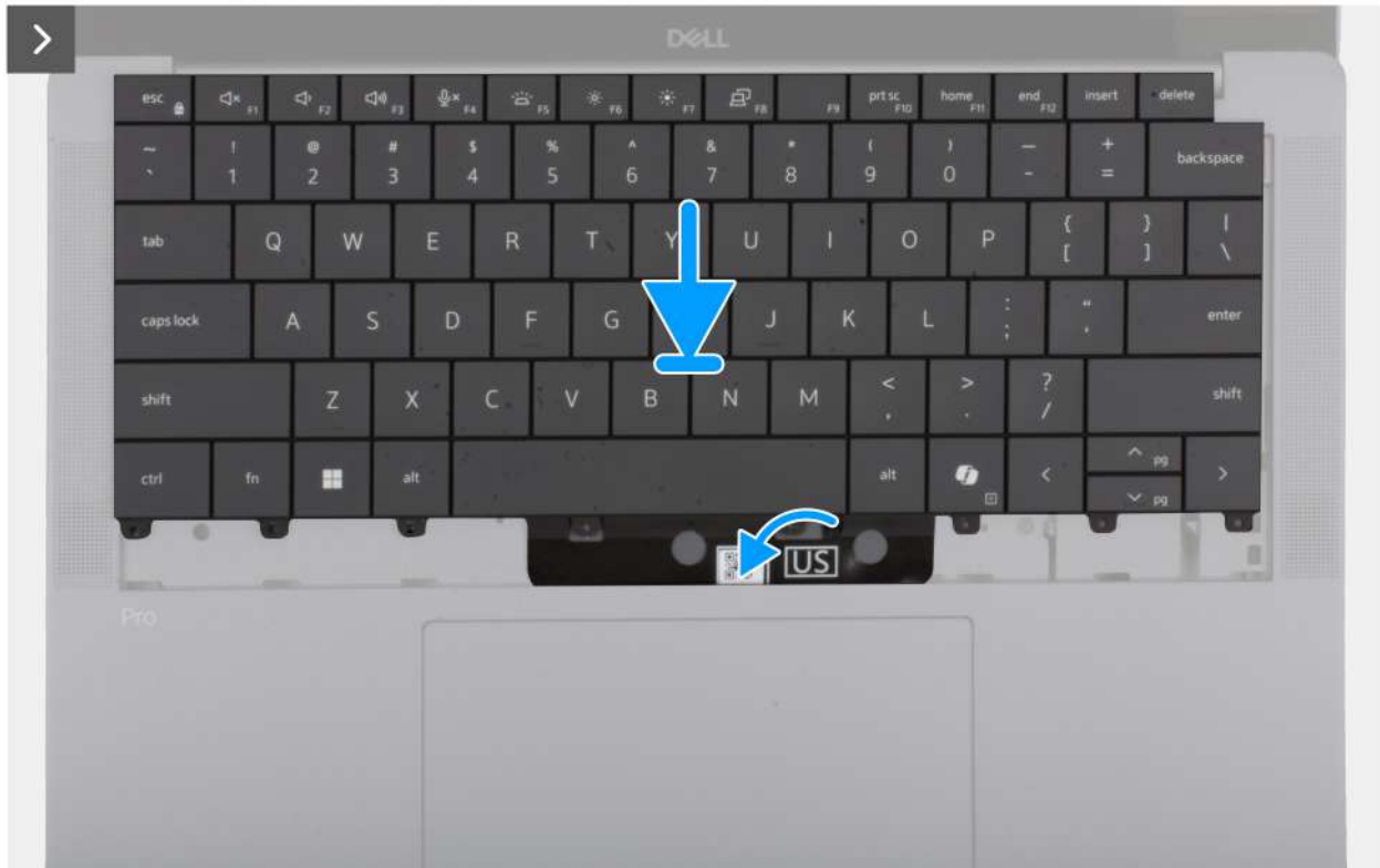
Figure 73. Installing the keyboard assembly
