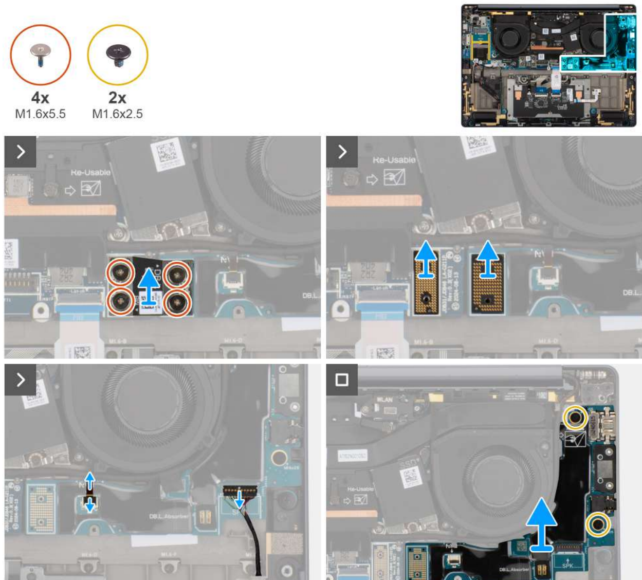
Figure 38. Removing the left I/O-board
